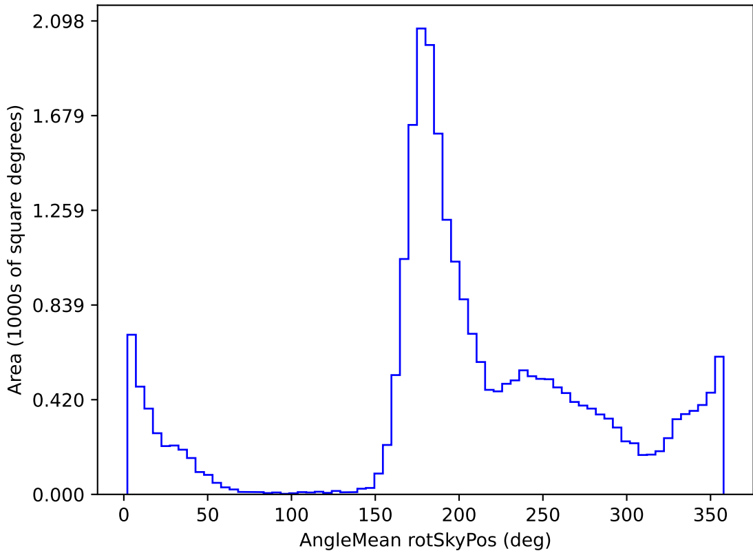
ddf_loaded_half_fl8_v3.4_10yrs All sky z band: AngleMean rotSkyPos
