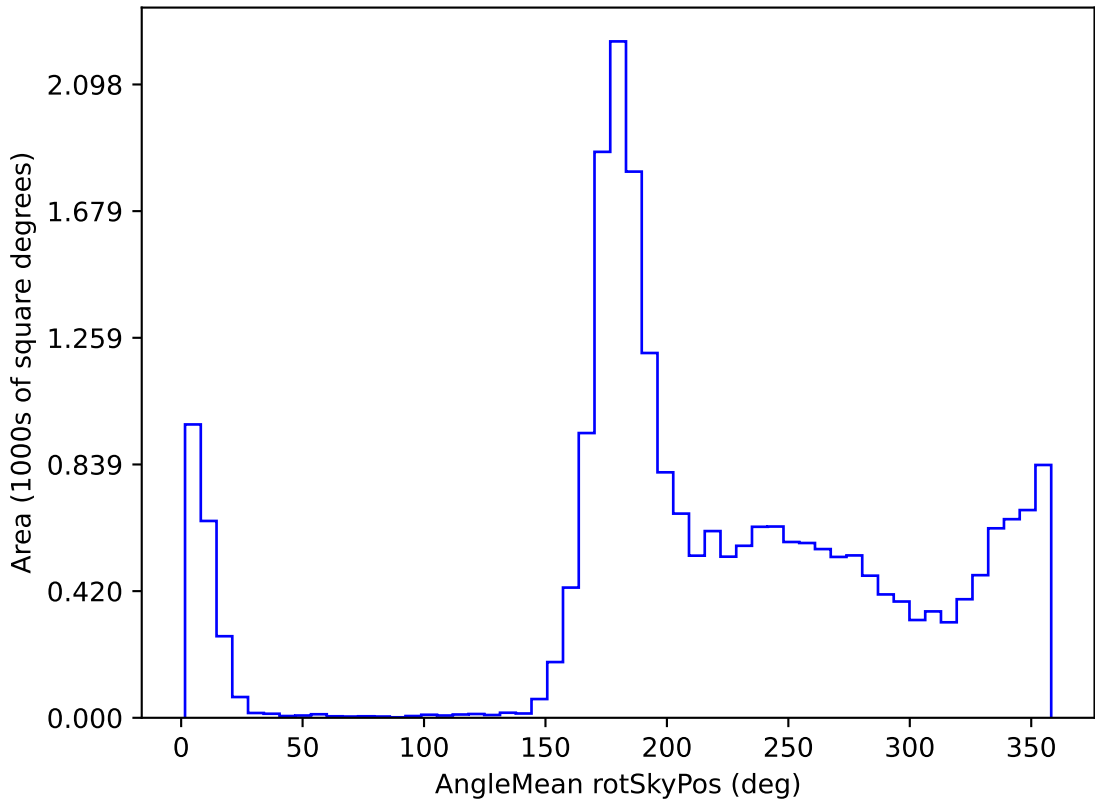
ddf_loaded_half_fl8_v3.4_10yrs All sky y band: AngleMean rotSkyPos
