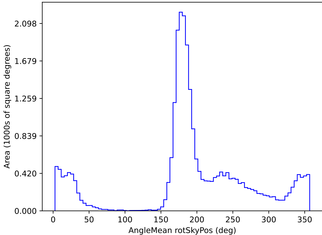
ddf_loaded_half_fl8_v3.4_10yrs All sky r band: AngleMean rotSkyPos
