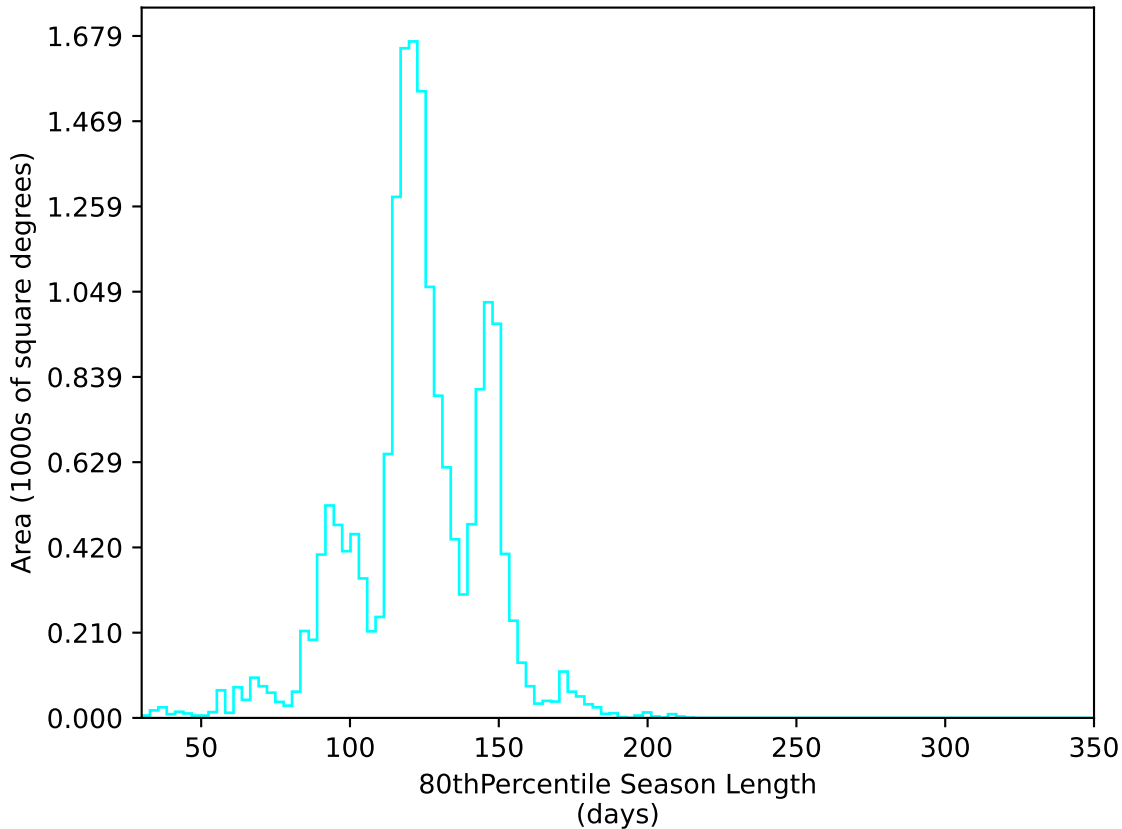
ddf_loaded_half_fl8_v3.4_10yrs WFD u band: 80thPercentile Season Length
