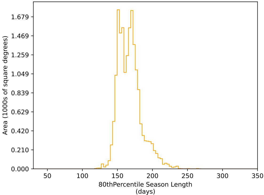
ddf_loaded_half_fl8_v3.4_10yrs WFD r band: 80thPercentile Season Length
