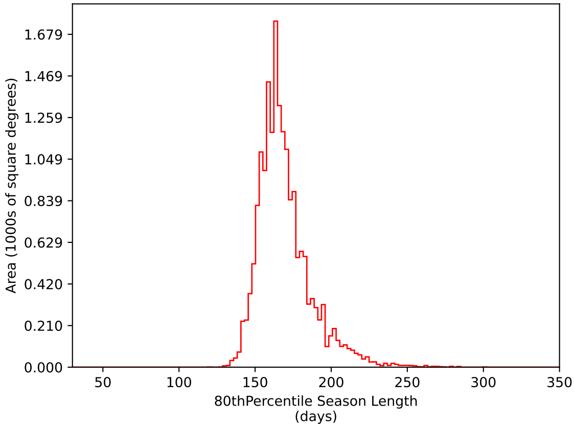
ddf_loaded_half_fl8_v3.4_10yrs WFD i band: 80thPercentile Season Length
