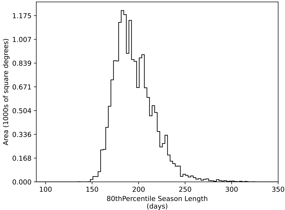
ddf_loaded_half_fl8_v3.4_10yrs WFD all bands: 80thPercentile Season Length
