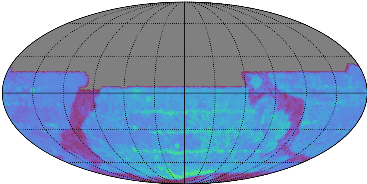
ddf_loaded_half_fl8_v3.4_10yrs All sky y band: 80thPercentile Season Length
