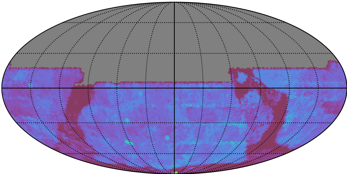
ddf_loaded_half_fl8_v3.4_10yrs All sky u band: 80thPercentile Season Length
