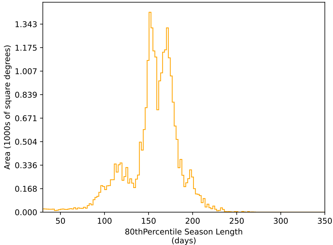
ddf_loaded_half_fl8_v3.4_10yrs All sky r band: 80thPercentile Season Length
