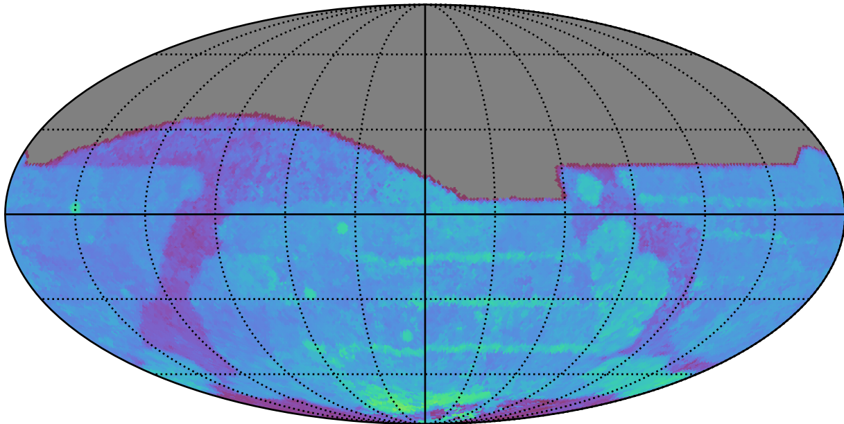
ddf_loaded_half_fl8_v3.4_10yrs All sky i band: 80thPercentile Season Length
