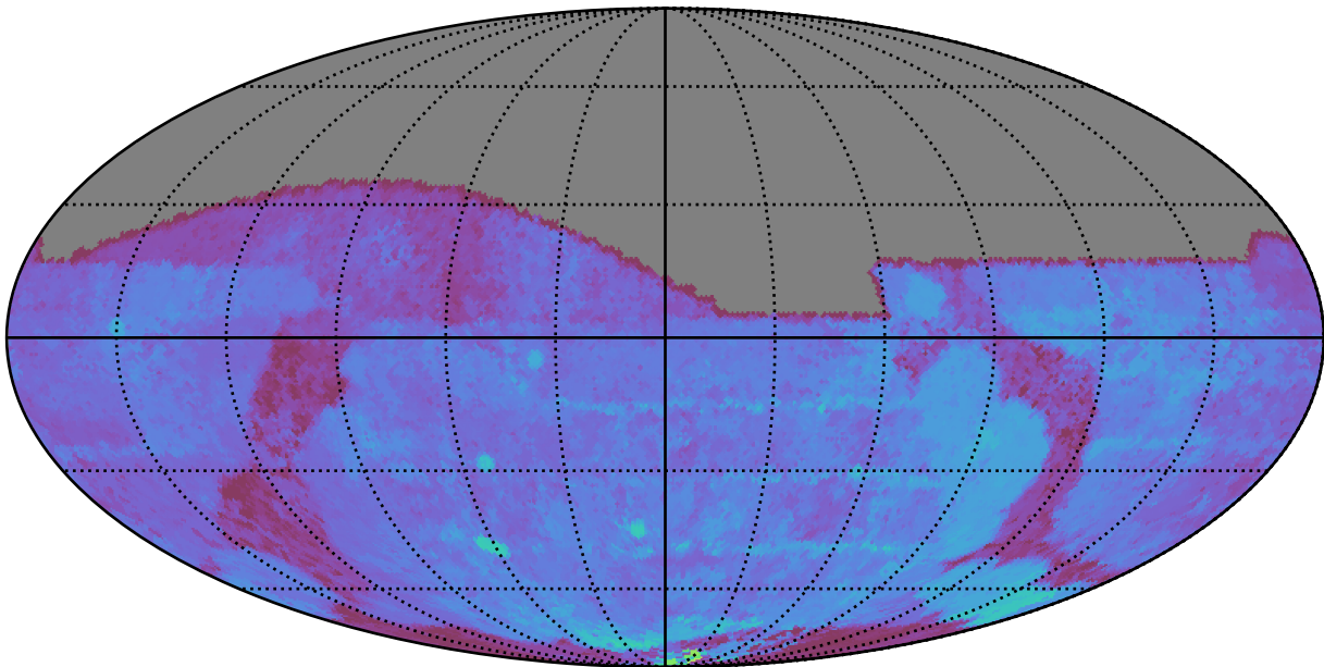
ddf_loaded_half_fl8_v3.4_10yrs All sky g band: 80thPercentile Season Length
