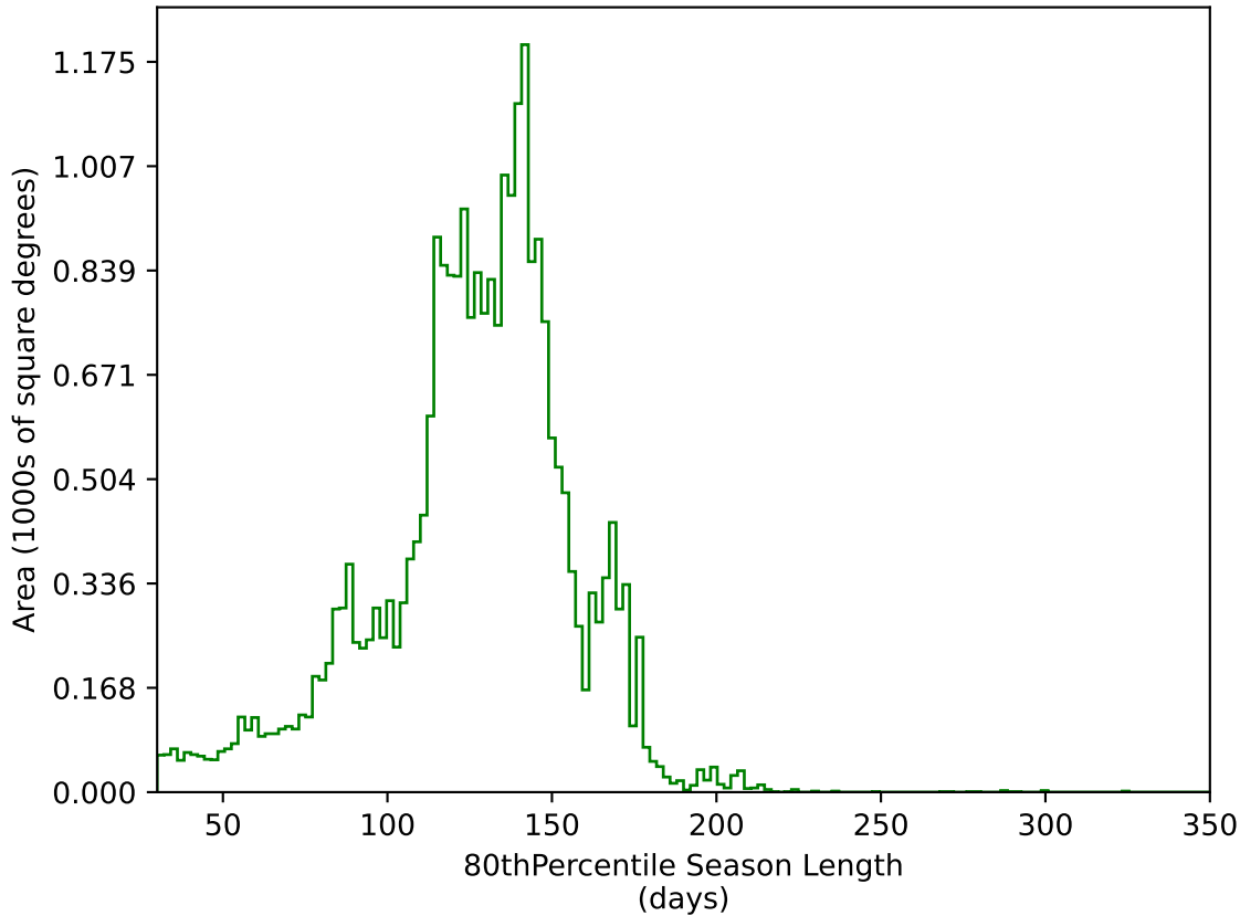
ddf_loaded_half_fl8_v3.4_10yrs All sky g band: 80thPercentile Season Length
