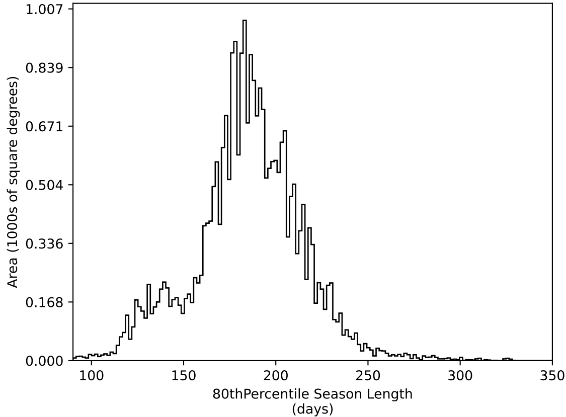
ddf_loaded_half_fl8_v3.4_10yrs All sky all bands: 80thPercentile Season Length
