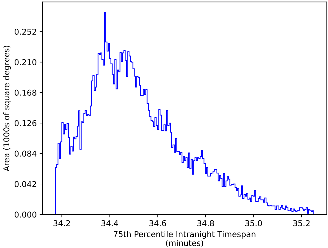
ddf_loaded_half_fl8_v3.4_10yrs WFD zy bands: 75th Percentile Intranight Timespan
