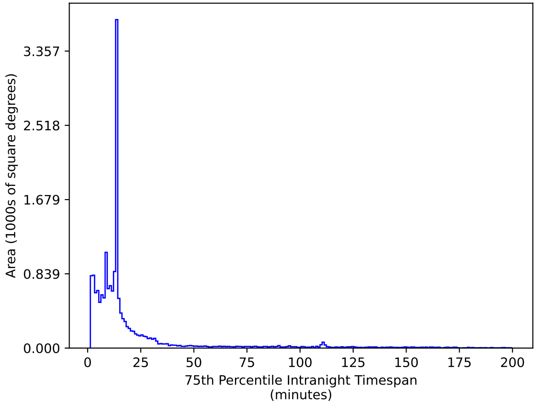
ddf_loaded_half_fl8_v3.4_10yrs WFD z band: 75th Percentile Intranight Timespan
