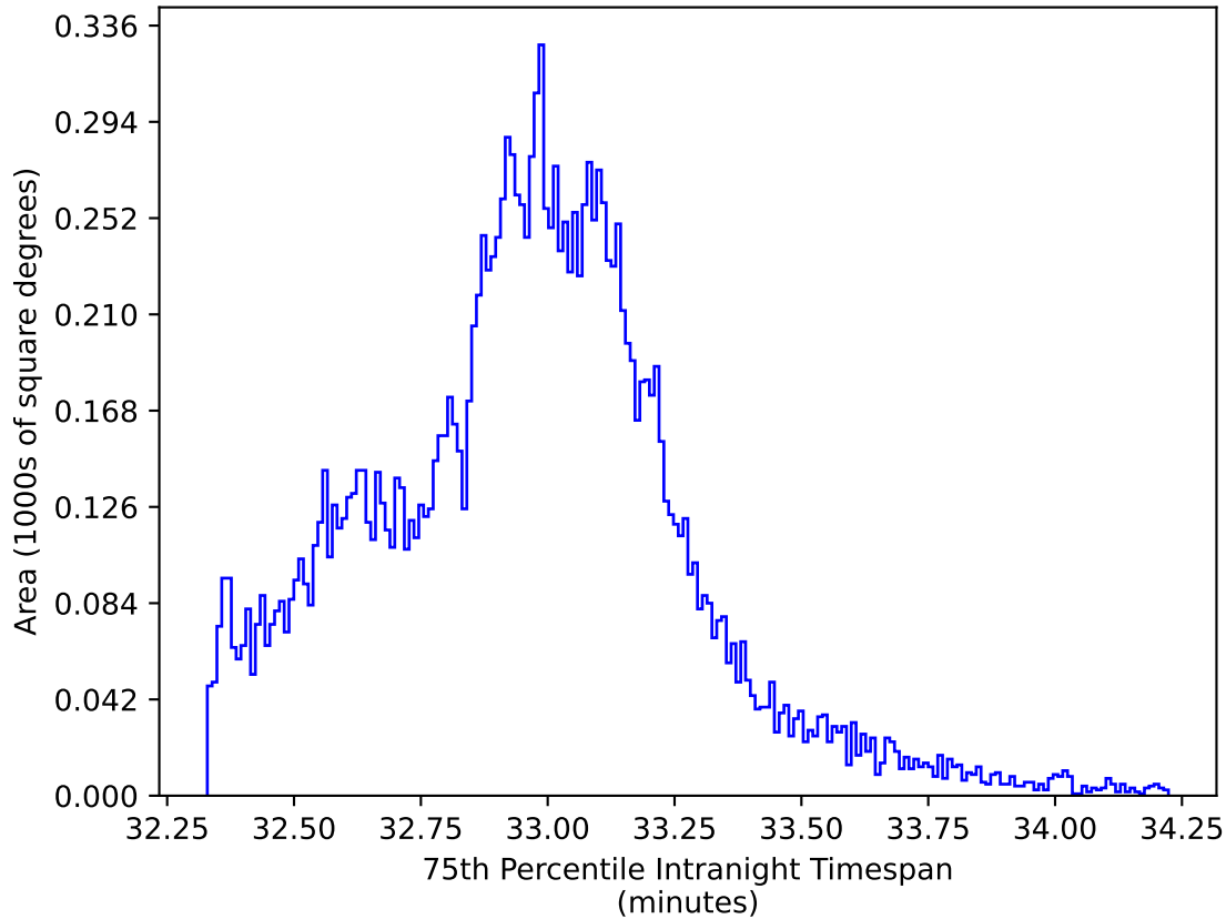
ddf_loaded_half_fl8_v3.4_10yrs WFD y band: 75th Percentile Intranight Timespan
