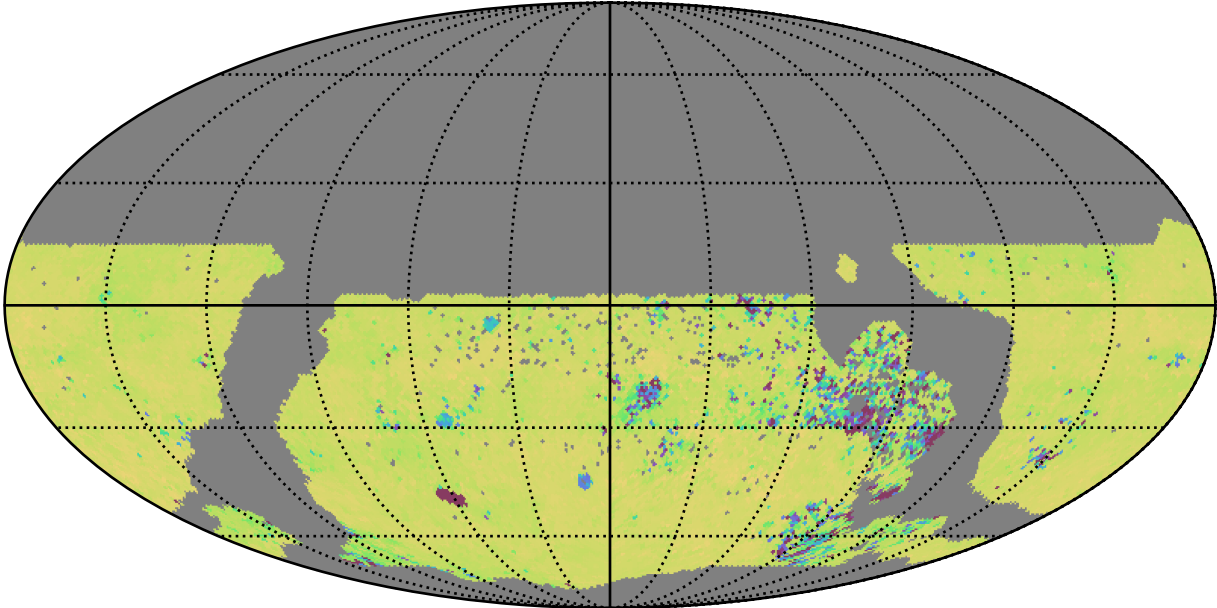
ddf_loaded_half_fl8_v3.4_10yrs WFD ug bands: 75th Percentile Intranight Timespan
