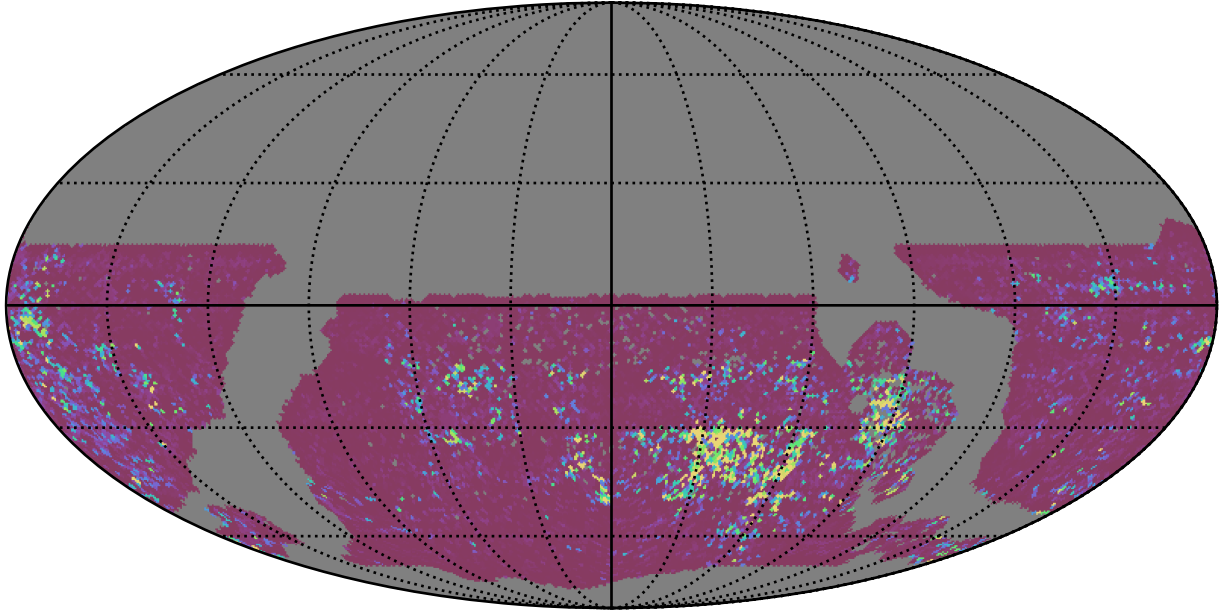
ddf_loaded_half_fl8_v3.4_10yrs WFD u band: 75th Percentile Intranight Timespan
