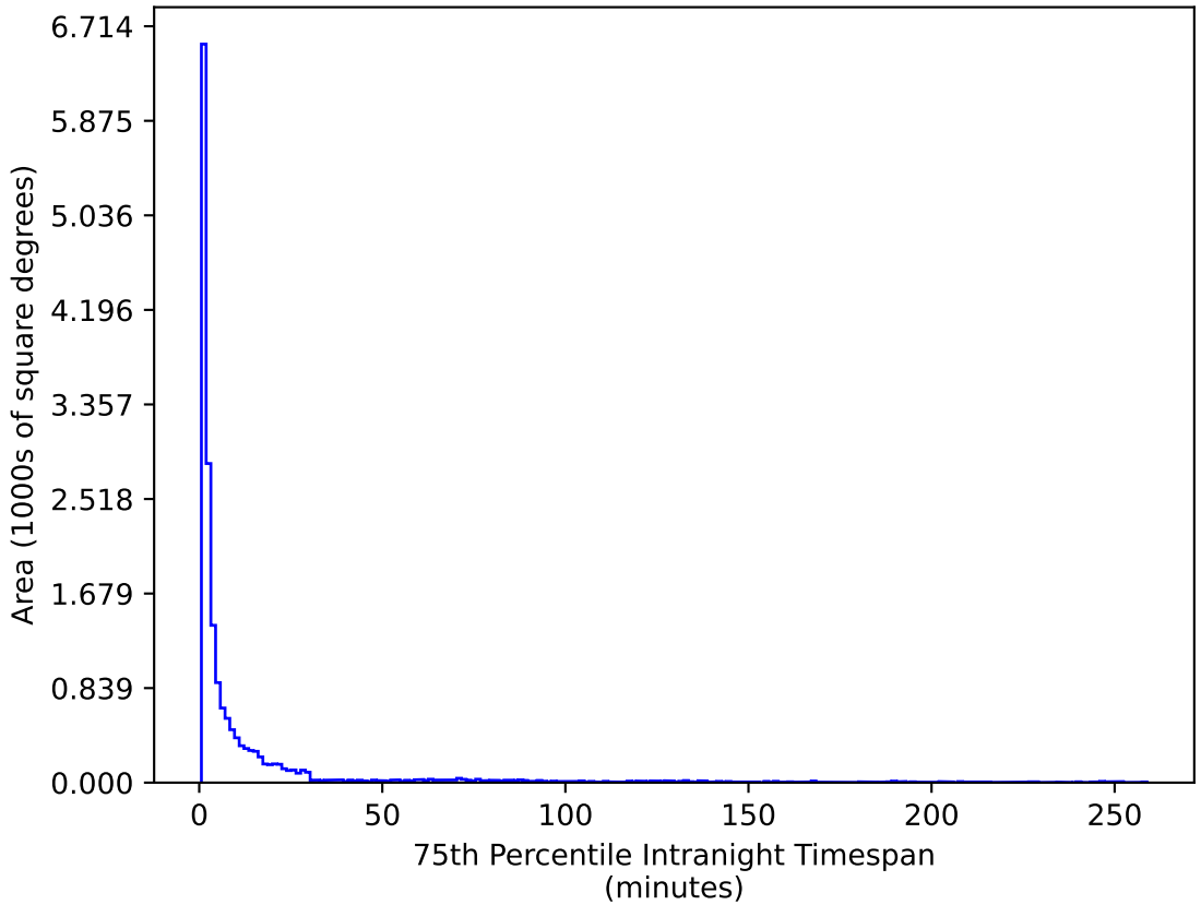
ddf_loaded_half_fl8_v3.4_10yrs WFD u band: 75th Percentile Intranight Timespan
