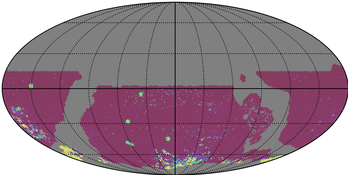
ddf_loaded_half_fl8_v3.4_10yrs WFD ri bands: 75th Percentile Intranight Timespan
