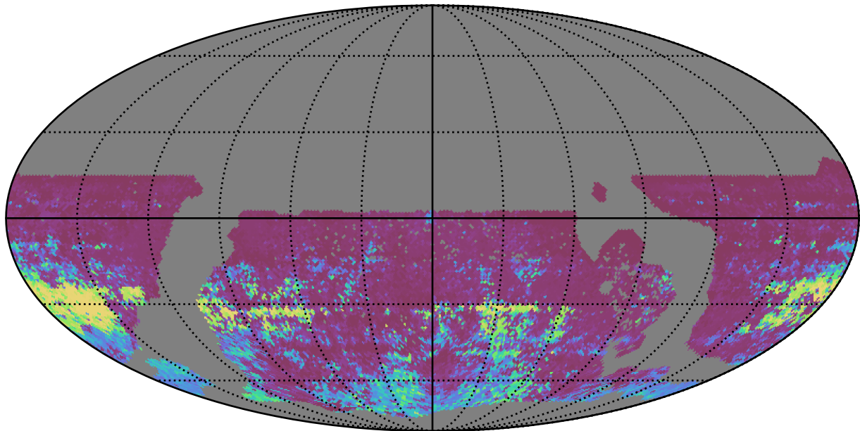
ddf_loaded_half_fl8_v3.4_10yrs WFD r band: 75th Percentile Intranight Timespan
