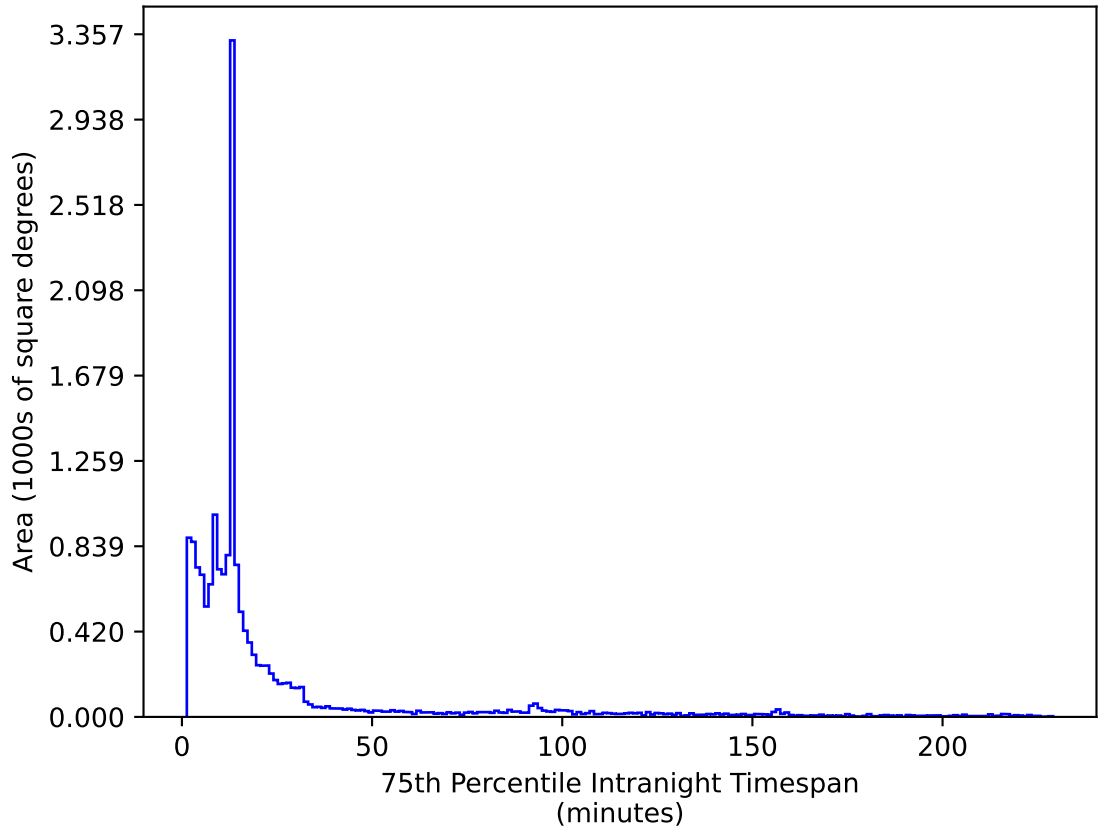
ddf_loaded_half_fl8_v3.4_10yrs WFD i band: 75th Percentile Intranight Timespan
