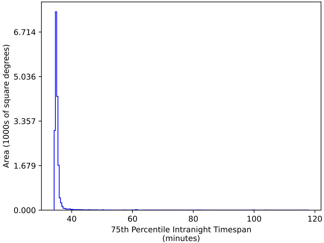
ddf_loaded_half_fl8_v3.4_10yrs WFD gr bands: 75th Percentile Intranight Timespan
