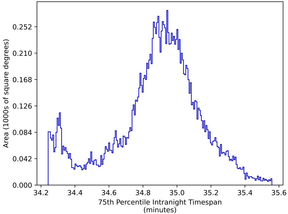
ddf_loaded_half_fl8_v3.4_10yrs WFD all bands: 75th Percentile Intranight Timespan
