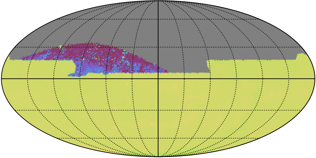
ddf_loaded_half_fl8_v3.4_10yrs All sky zy bands: 75th Percentile Intranight Timespan
