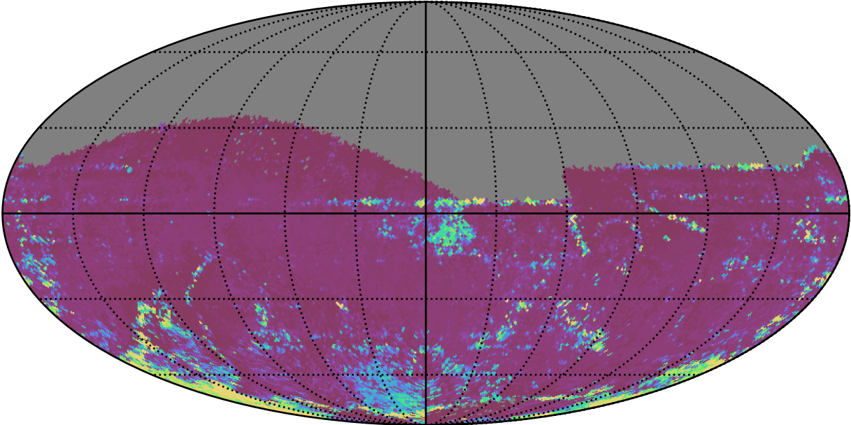
ddf_loaded_half_fl8_v3.4_10yrs All sky z band: 75th Percentile Intranight Timespan
