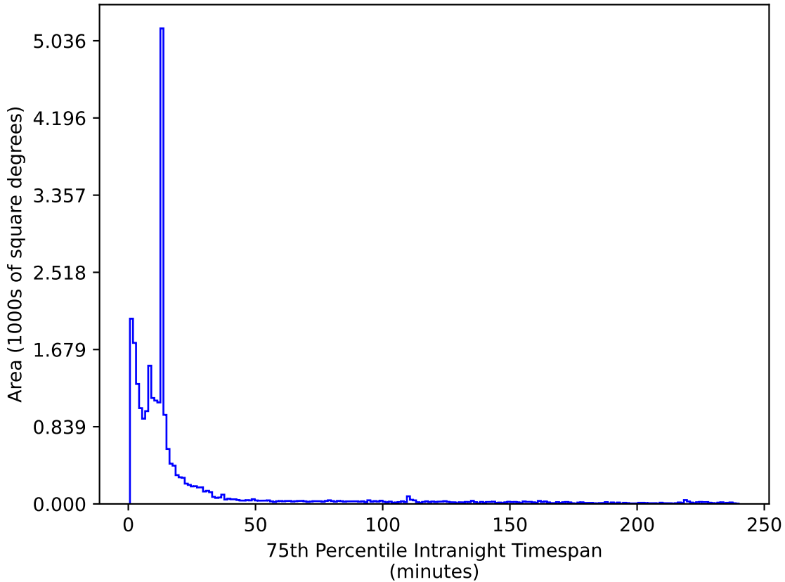
ddf_loaded_half_fl8_v3.4_10yrs All sky z band: 75th Percentile Intranight Timespan
