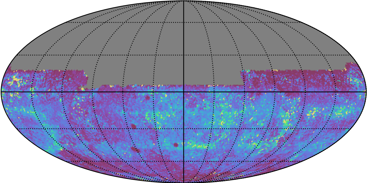
ddf_loaded_half_fl8_v3.4_10yrs All sky y band: 75th Percentile Intranight Timespan
