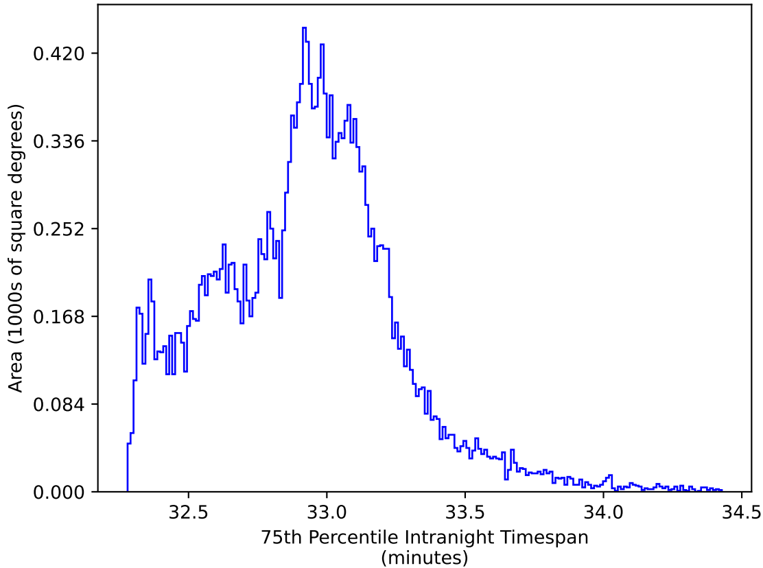
ddf_loaded_half_fl8_v3.4_10yrs All sky y band: 75th Percentile Intranight Timespan
