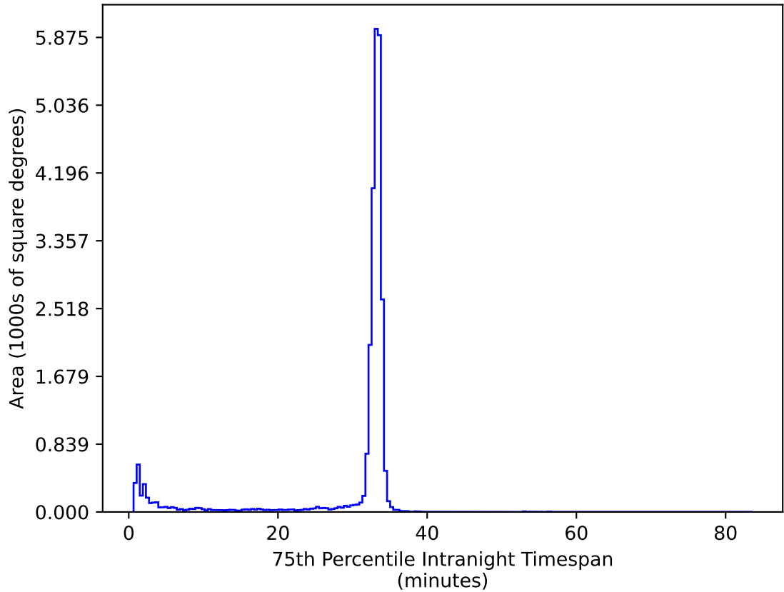
ddf_loaded_half_fl8_v3.4_10yrs All sky ug bands: 75th Percentile Intranight Timespan
