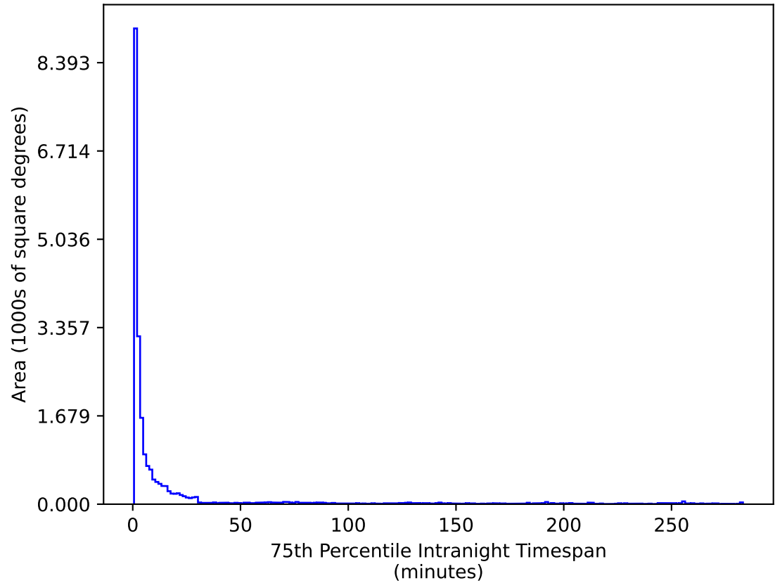
ddf_loaded_half_fl8_v3.4_10yrs All sky u band: 75th Percentile Intranight Timespan
