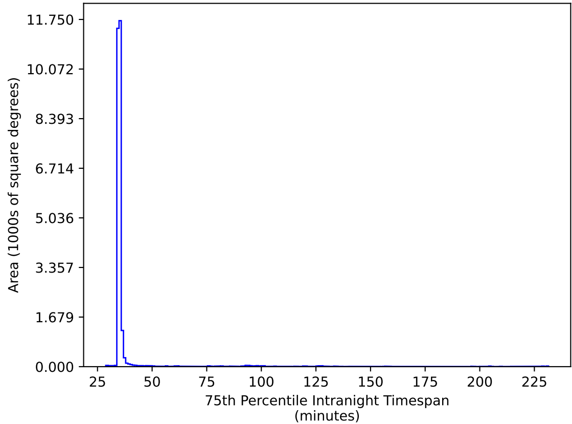
ddf_loaded_half_fl8_v3.4_10yrs All sky ri bands: 75th Percentile Intranight Timespan
