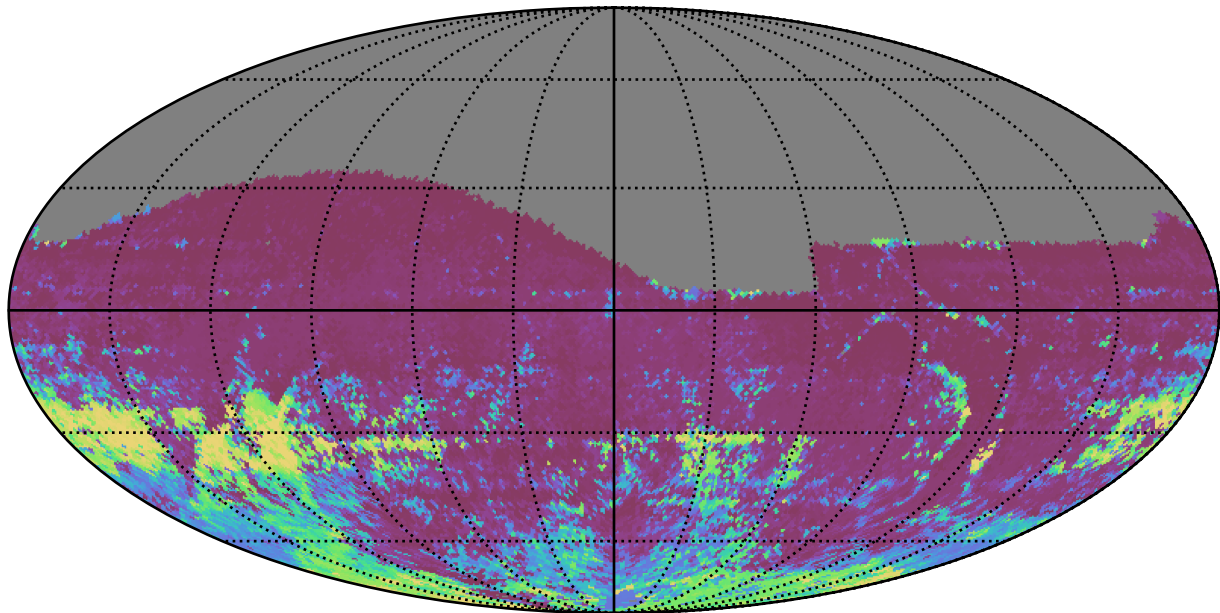
ddf_loaded_half_fl8_v3.4_10yrs All sky r band: 75th Percentile Intranight Timespan
