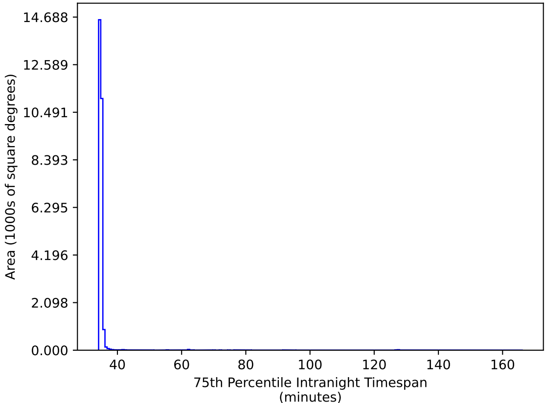
ddf_loaded_half_fl8_v3.4_10yrs All sky iz bands: 75th Percentile Intranight Timespan
