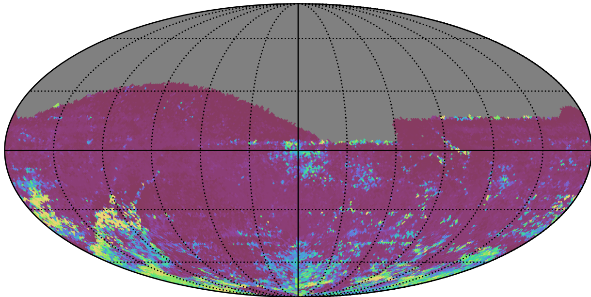
ddf_loaded_half_fl8_v3.4_10yrs All sky i band: 75th Percentile Intranight Timespan
