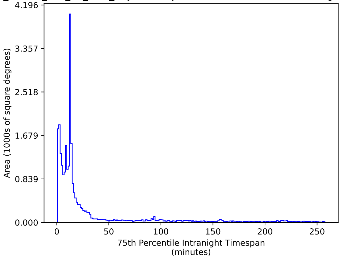
ddf_loaded_half_fl8_v3.4_10yrs All sky i band: 75th Percentile Intranight Timespan
