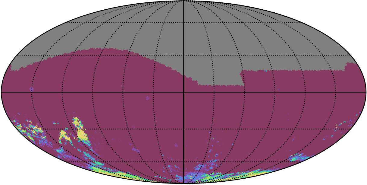
ddf_loaded_half_fl8_v3.4_10yrs All sky gr bands: 75th Percentile Intranight Timespan
