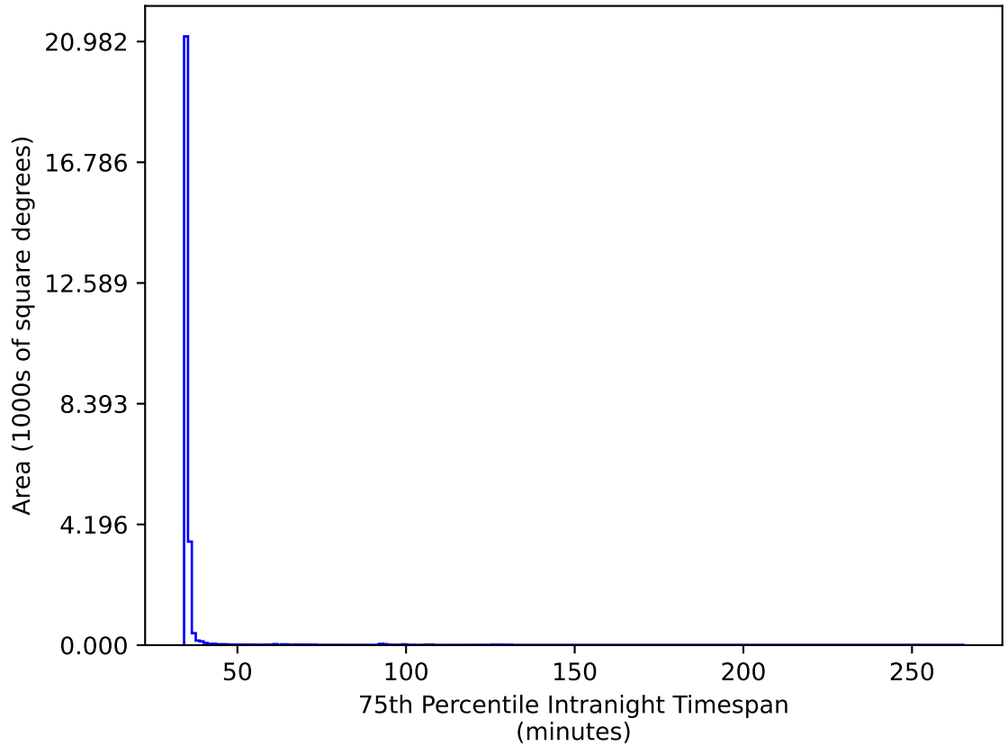
ddf_loaded_half_fl8_v3.4_10yrs All sky gr bands: 75th Percentile Intranight Timespan
