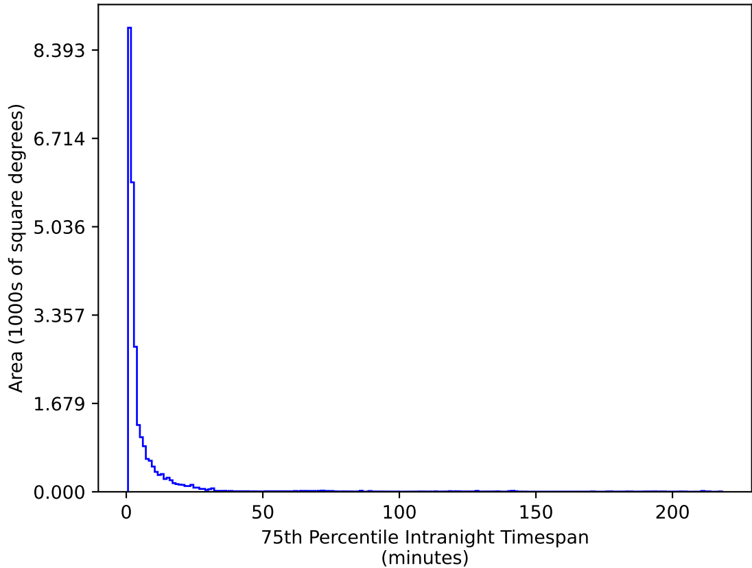
ddf_loaded_half_fl8_v3.4_10yrs All sky g band: 75th Percentile Intranight Timespan
