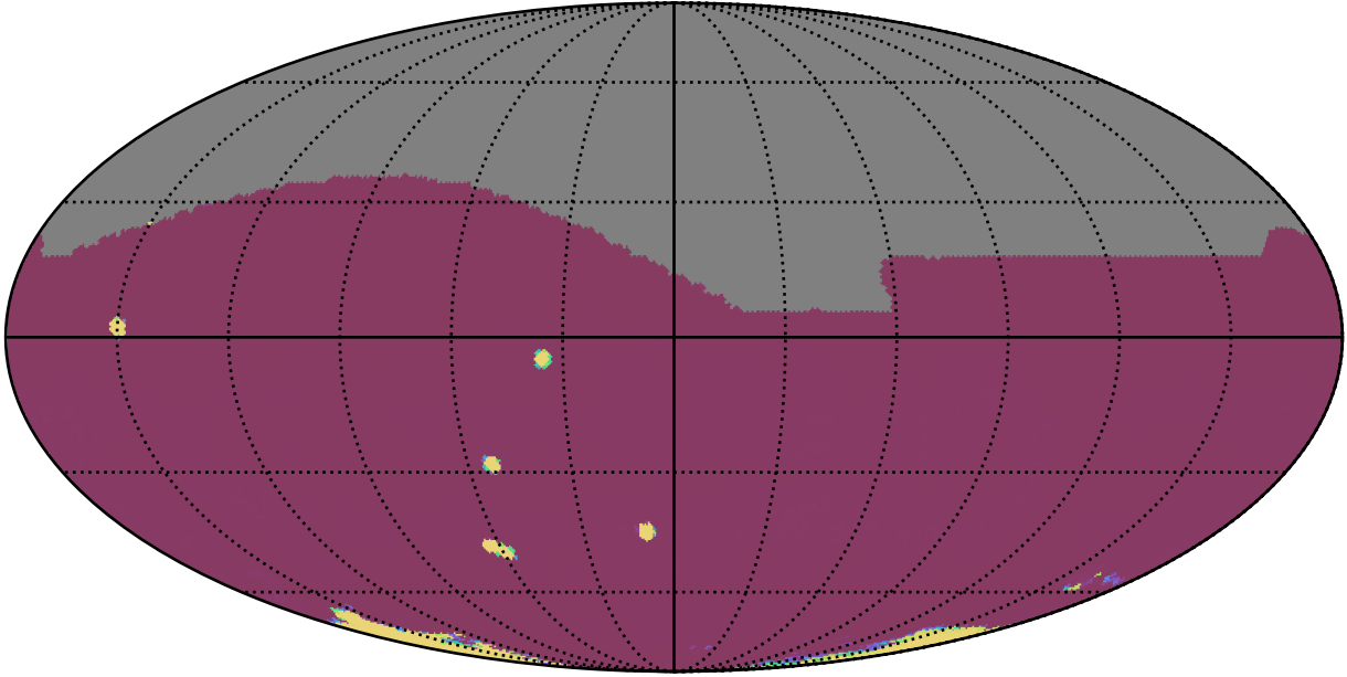
ddf_loaded_half_fl8_v3.4_10yrs All sky all bands: 75th Percentile Intranight Timespan
