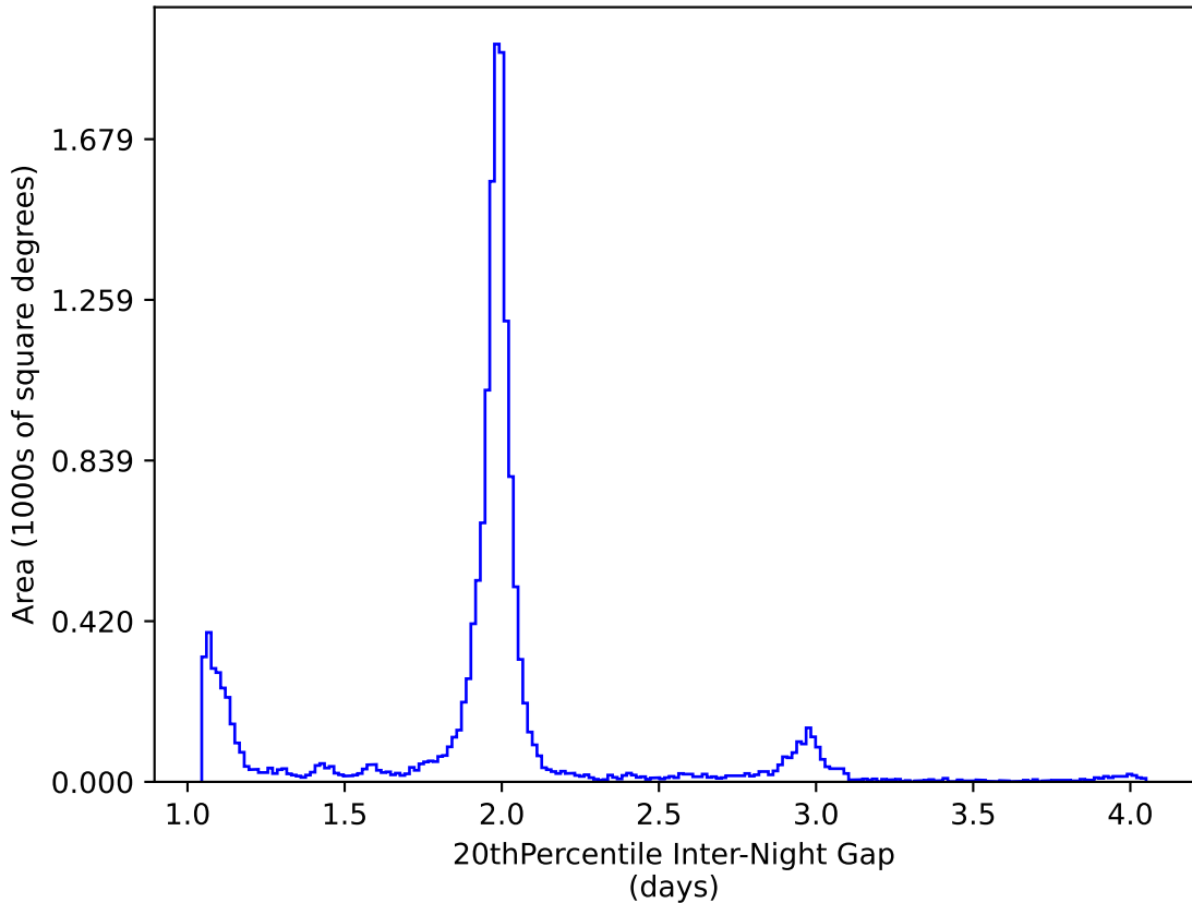
ddf_loaded_half_fl8_v3.4_10yrs WFD y band: 20thPercentile Inter-Night Gap
