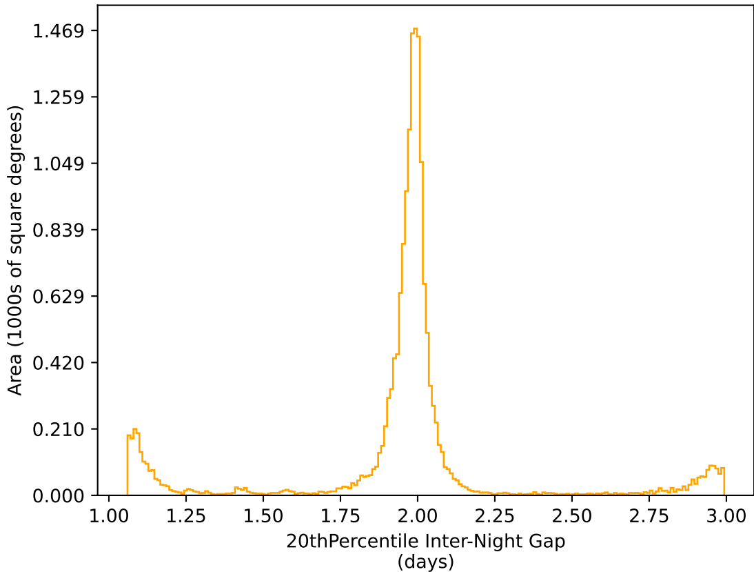
ddf_loaded_half_fl8_v3.4_10yrs WFD r band: 20thPercentile Inter-Night Gap
