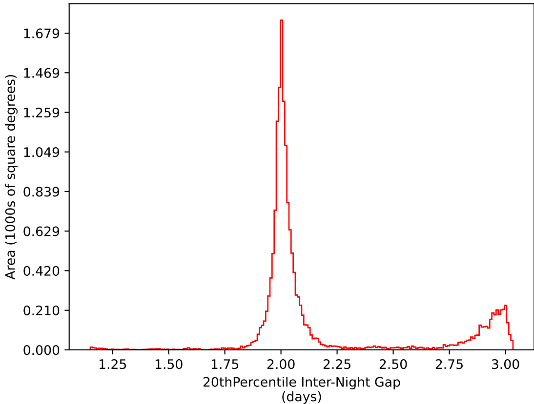
ddf_loaded_half_fl8_v3.4_10yrs WFD i band: 20thPercentile Inter-Night Gap
