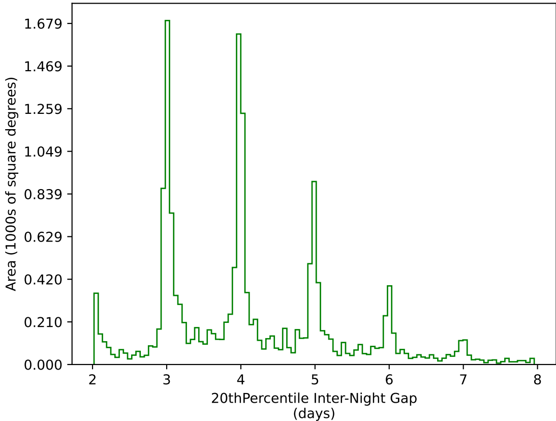
ddf_loaded_half_fl8_v3.4_10yrs WFD g band: 20thPercentile Inter-Night Gap
