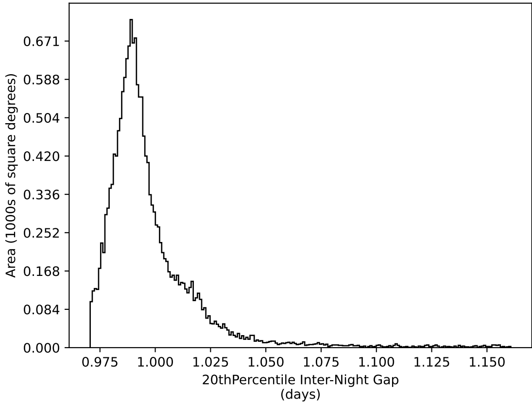
ddf_loaded_half_fl8_v3.4_10yrs WFD all bands: 20thPercentile Inter-Night Gap
