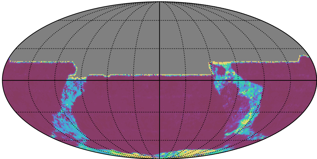
ddf_loaded_half_fl8_v3.4_10yrs All sky y band: 20thPercentile Inter-Night Gap
