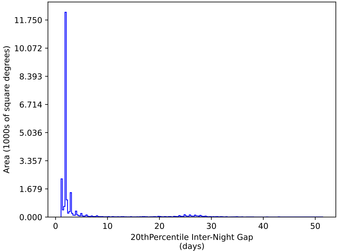
ddf_loaded_half_fl8_v3.4_10yrs All sky y band: 20thPercentile Inter-Night Gap
