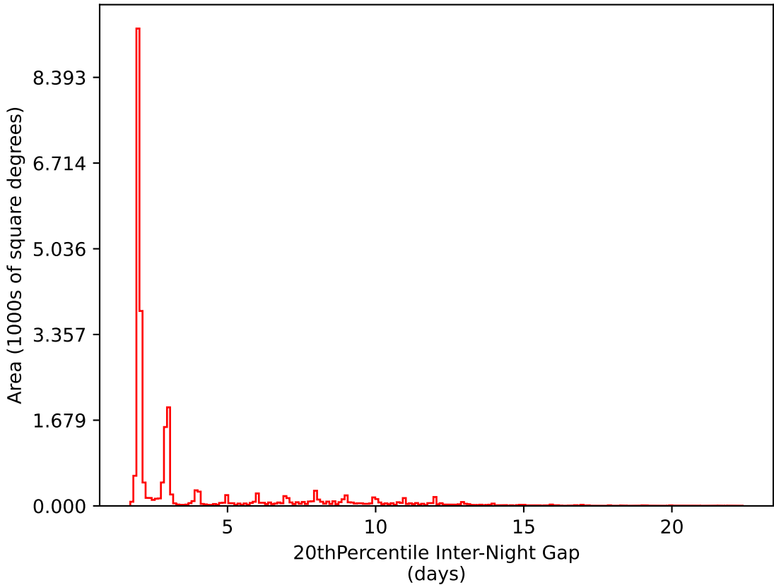
ddf_loaded_half_fl8_v3.4_10yrs All sky i band: 20thPercentile Inter-Night Gap
