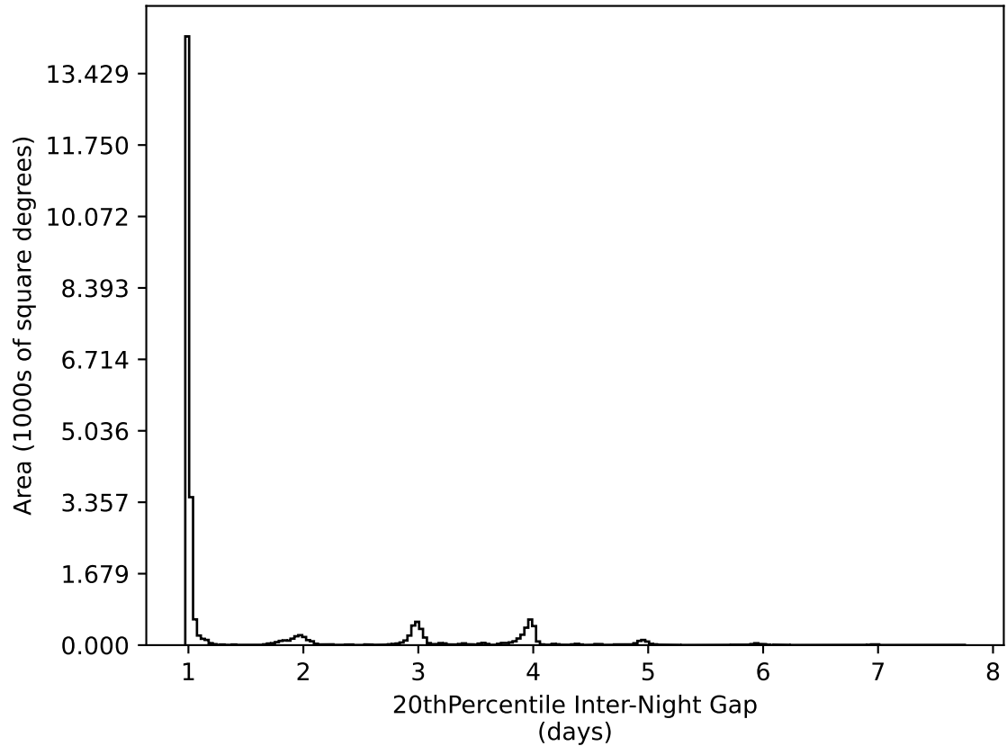
ddf_loaded_half_fl8_v3.4_10yrs All sky all bands: 20thPercentile Inter-Night Gap
